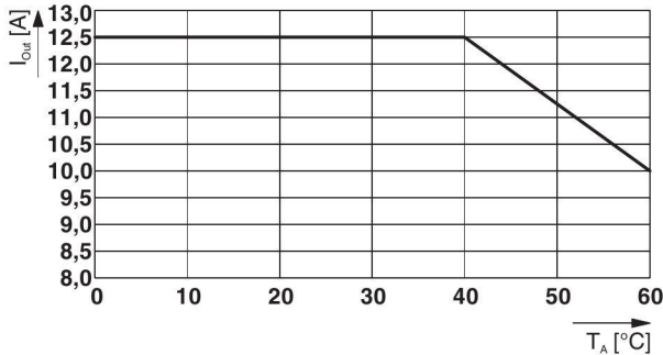
Figure 29 Temperature-dependent derating
