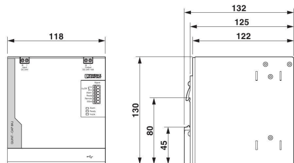
Figure 3 Device dimensions
