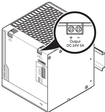
Figure 12 Connection terminal blocks output voltage: Output +/-
