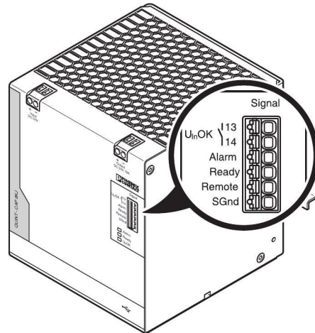
Figure 13 Signal inputs and outputs
