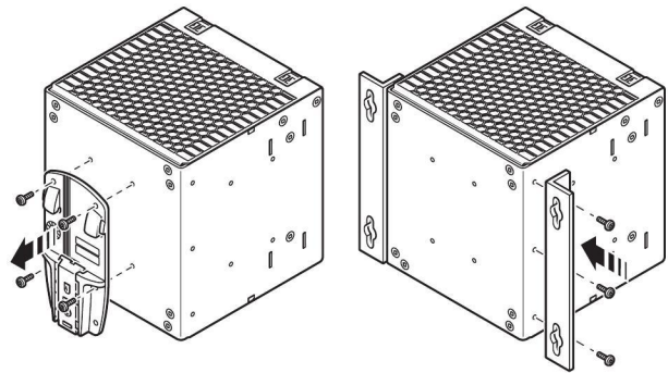
Figure 10 Mounting the UWA 130 universal wall adapter
