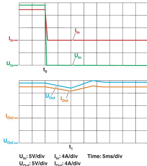
Figure 32 Switching behavior
