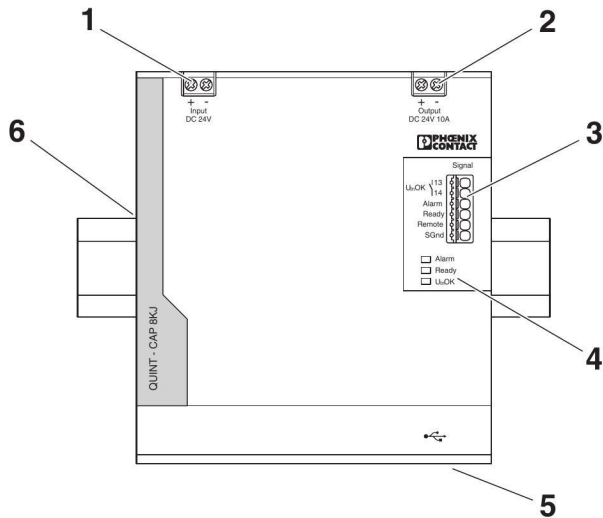
Figure 1 Position of the function elements
