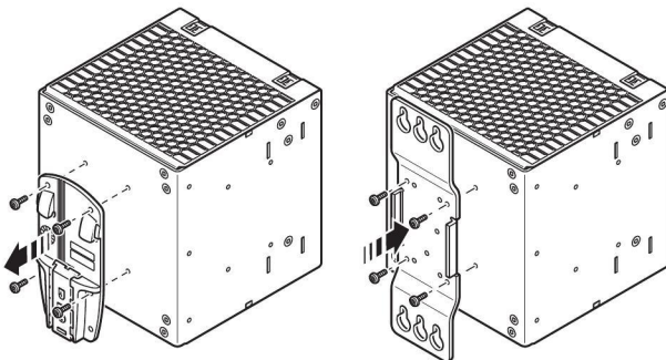
Figure 9 Mounting the UWA 182/52 universal wall adapter
