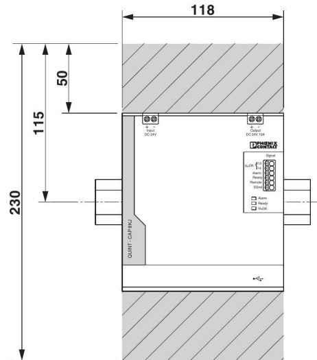
Figure 2 Keep-out areas
